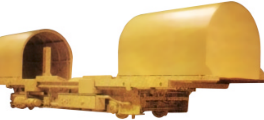
70 Ton capacity, radio controlled, battery powered, steel coil transfer car with motor operated environmental protection covers
