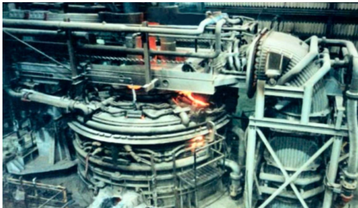
40 Ton special application steel furnace
